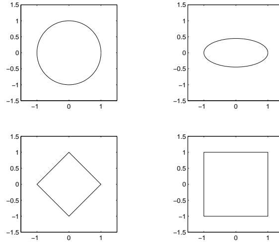
Figure 7.5 The balls B(0, 1) in Exercise 4.1
