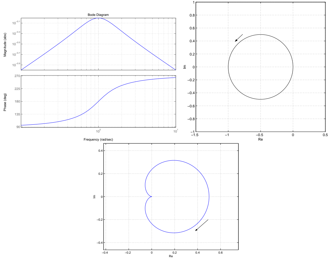
Figure 4.5 Bode and Nyquist curves for the system in Exercise 4.6a (above) and Nyquist curve for the system in Exercise 4.6b (below)
