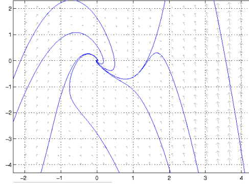
Figure 7.18 Phase plane for system in exercise 7.22.
