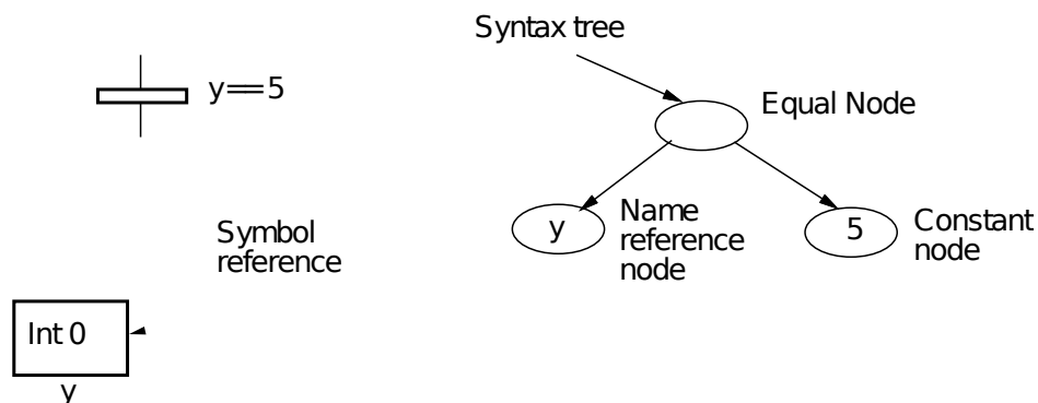
Figure 1.8: Syntax tree for the expression y = 5 .
