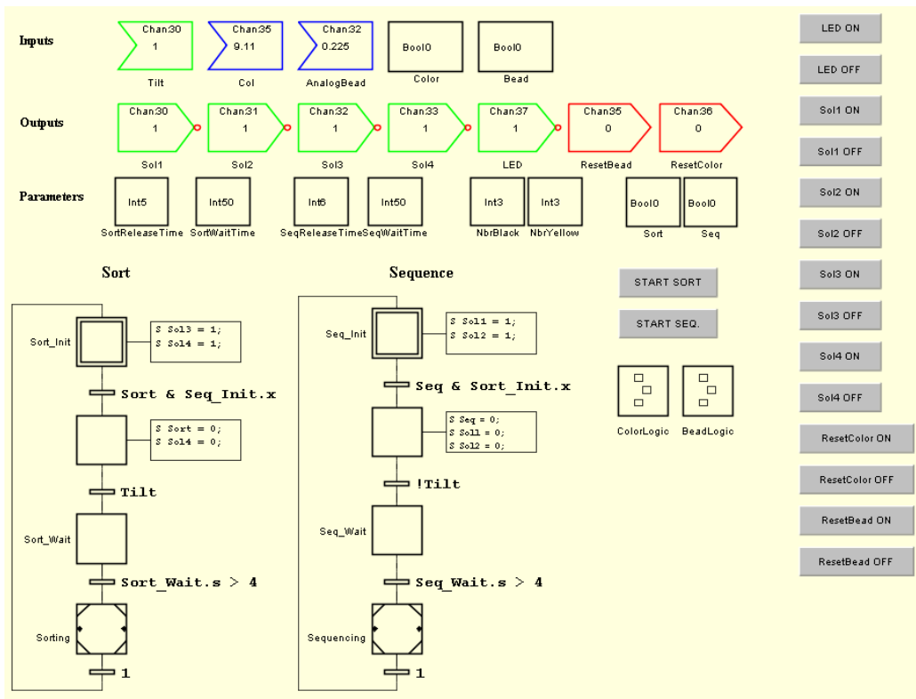
Figure 2.2: The template Grafchart.
