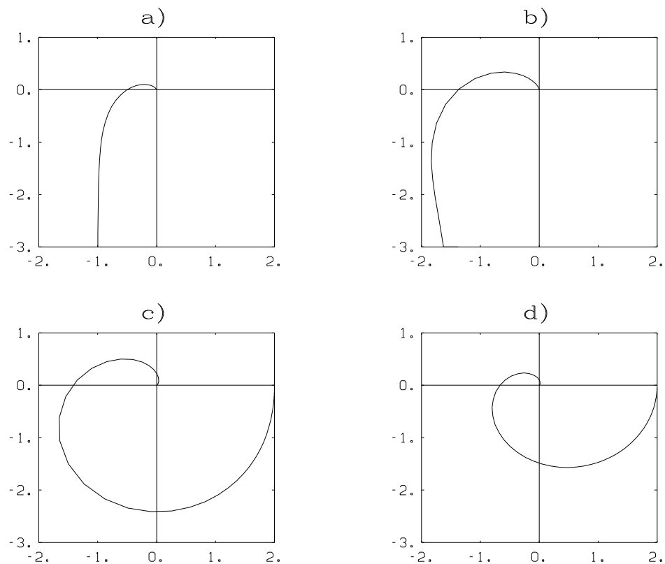
Figure 4.1 Nyquist curves in assignment 4.12.
