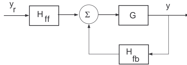
Figure 7.4 Equivalent block diagram in assignment 7.3.
