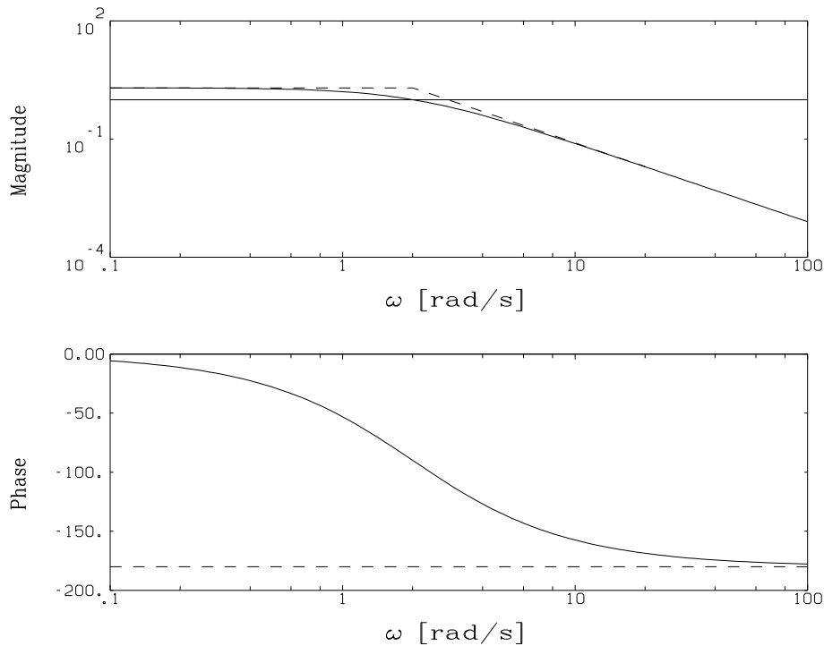
Figure 6.9 Bode plot of the system in assignment 6.11.
