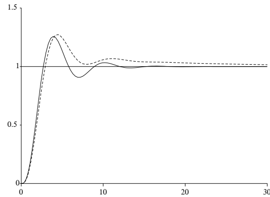
Figure 6.16 Step response of the uncompensated closed loop system (solid line) as well as the compensated closed loop system (dashed line) in assignment 6.16.
