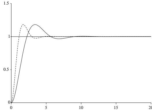
Figure 6.8 Step response of the uncompensated closed loop system (solid line) as well as the compensated closed loop system (dashed line) in assignment 6.13.
