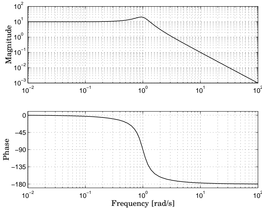
Figure 3.4 The Bode plot of the oscillating mass in assignment 3.3.
