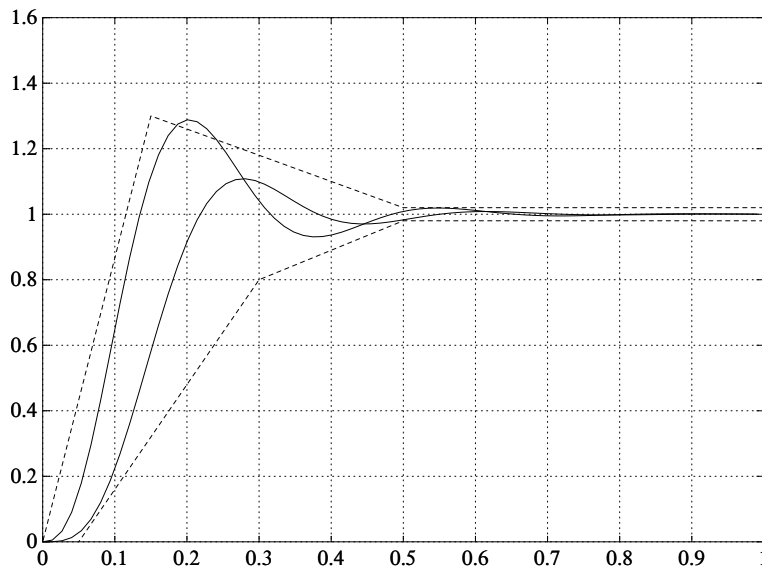
Figure 8.10 Step response of the closed loop system for \omega_m = 20 rad/s. Choosing L_r according to sub-assignment b yields the system with the larger overshoot. The other curve is the step response corresponding to L_r = 0 .
