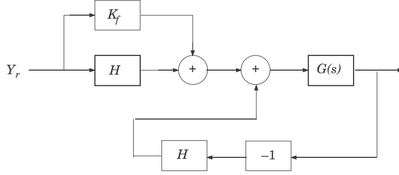
Figure 7.2 Modified block diagram in assignment 7.3.
