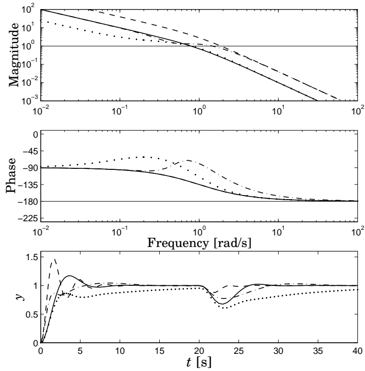
Figure 6.1 Bode plot and step response for the case when the PID parameters in sub-assignment 6.2b have been multiplied by four. The solid curves correspond to the nominal case.
