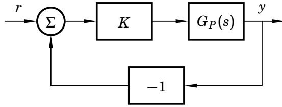
Figure 4.3 The closed loop system in assignment 4.17.
