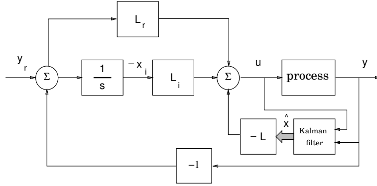
Figure 8.8 Block diagram showing the Kalman filter and state feedback in assignment 8.2.
