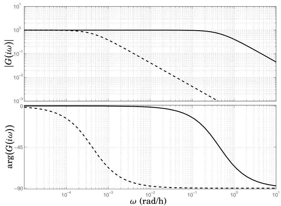
Figure 3.3 Bode diagram in problem 3.2.
