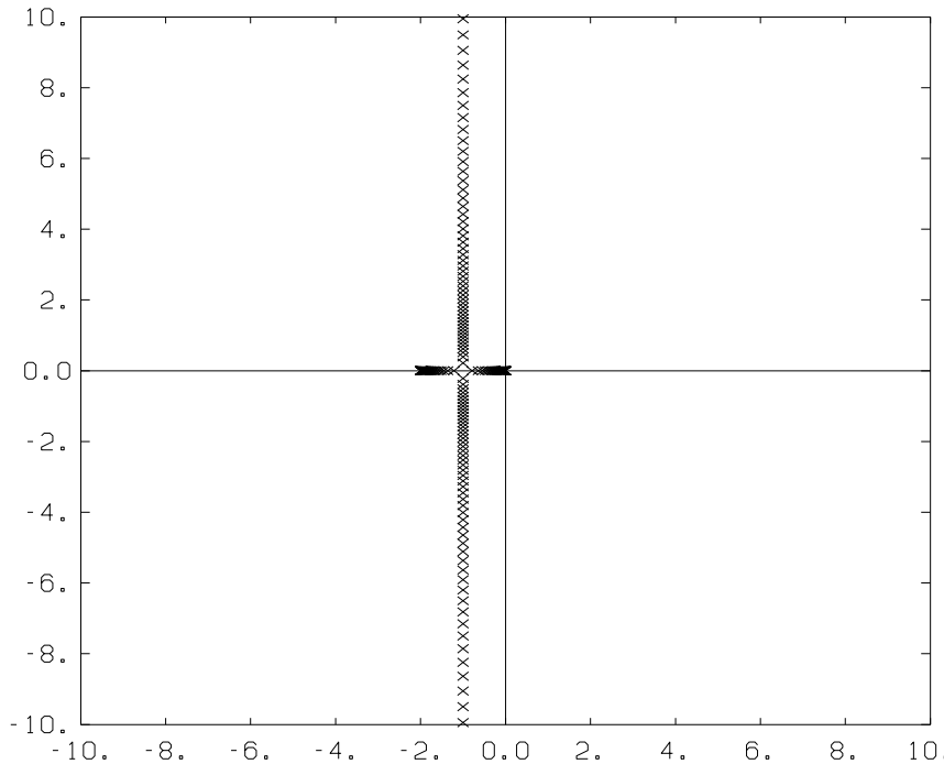
Figure 4.1 Root locus of the system in assignment 4.9.
