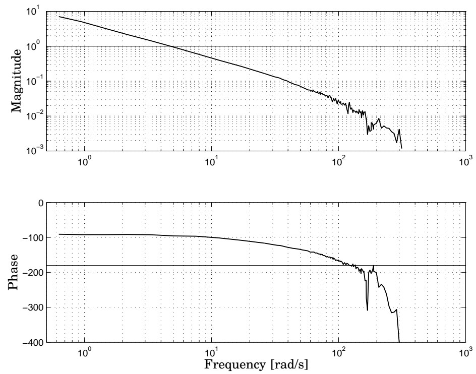
Figure 7.9 Measured Bode plot of the beam.
