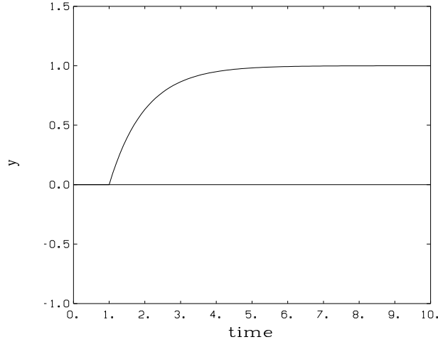
Figure 6.3 Step response of G(s) = e^{-s}/(s+1) .
