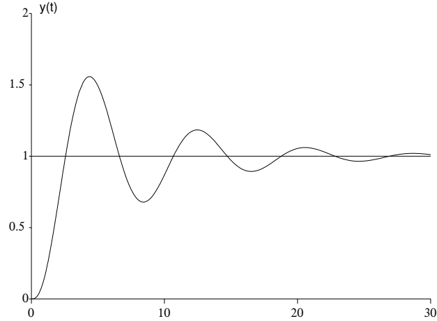
Figure 6.10 Step response of the closed loop servo system in assignment 6.15.
