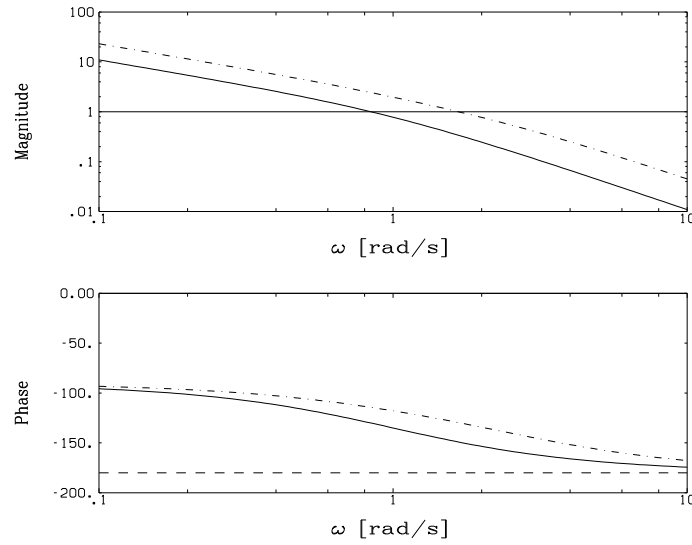
Figure 6.7 Bode plot of the uncompensated open loop system (solid line) as well as the compensated open loop system (dash-dotted line) in assignment 6.13.
