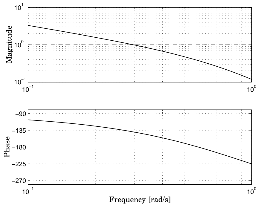
Figure 4.5 Bode plot of the open loop system in Figure 4.18.
