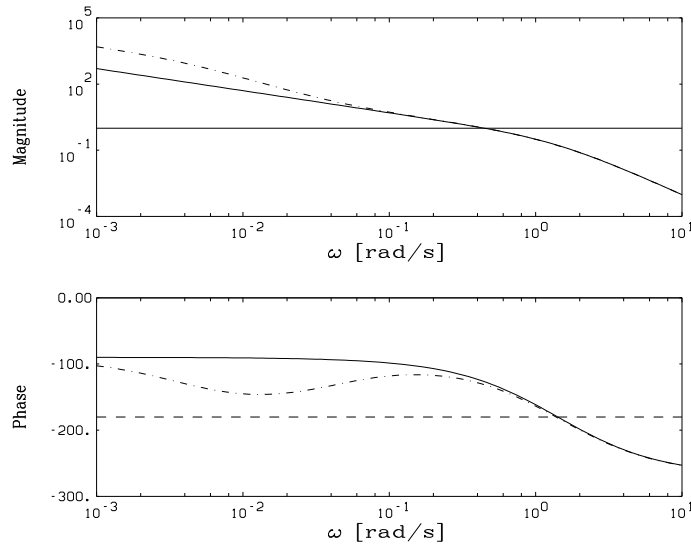
Figure 6.4 Bode plot of the uncompensated open loop system (solid line) and compensated open loop system (dash-dotted line) in assignment 6.12. K = 1 for both cases.
