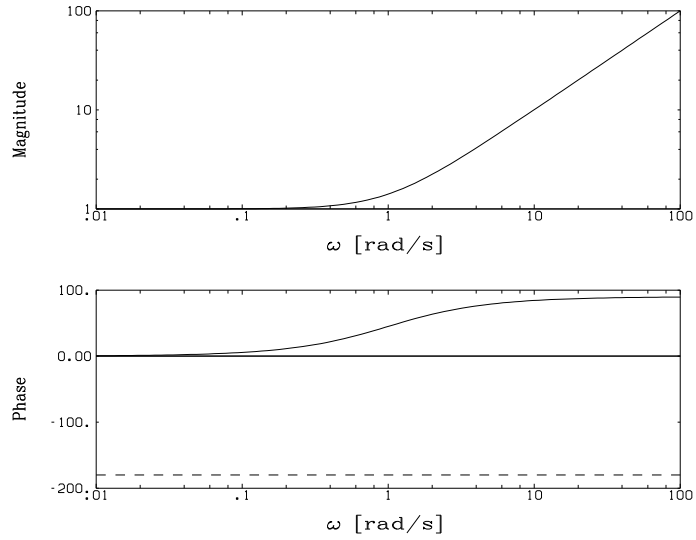
Figure 6.2 Bode plot of a PD controller with K = 1 and T_d = 1 .
