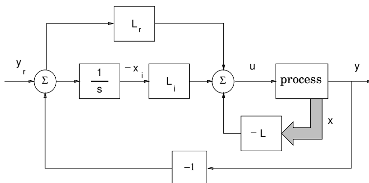
Figure 8.7 Block diagram of the state feedback control system in assignment 8.2.
