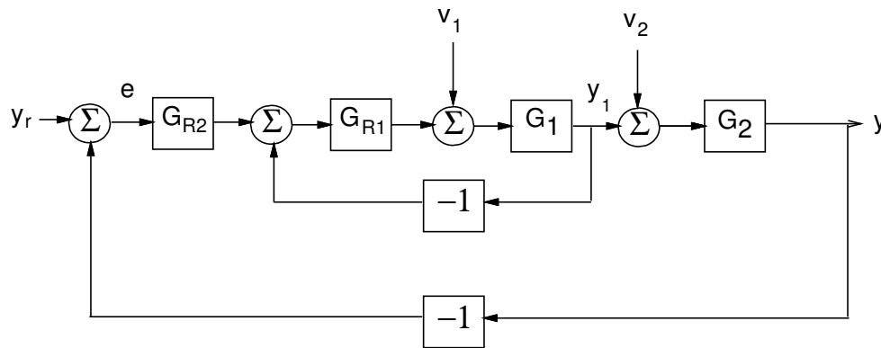
Figure 7.5 The cascade in assignment 7.5.
