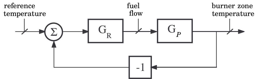
Figure 6.3 Block diagram of a cement oven with temperature controller.
