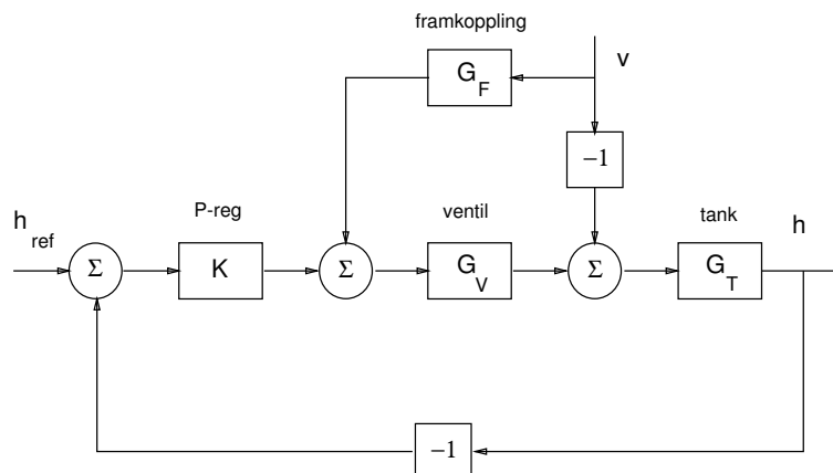
Figure 7.2 Block diagram of the level control system in assignment 7.2.
