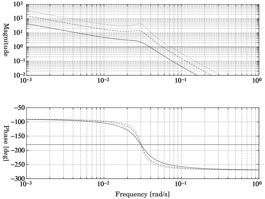
Figure 8.2 Bode plot of the estimated transfer function G(s) from \beta [deg] to h [m] in assignment 8.1 for the speeds v = 3 (solid curves), 5 (dashed curves) and 7 knots (dotted curves).
