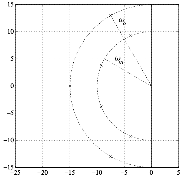
Figure 8.9 The pole placement in assignment 8.2.
