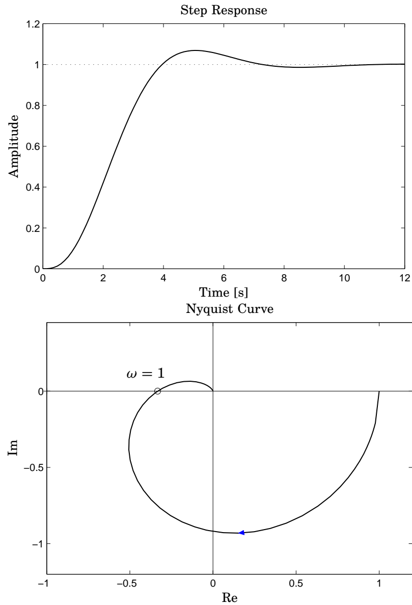
Figure 6.5 Step response and Nyquist curve of the system in assignment 6.8.
