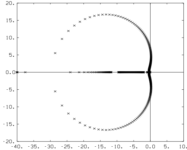
Figure 4.2 Root locus of the system in assignment 4.10.
