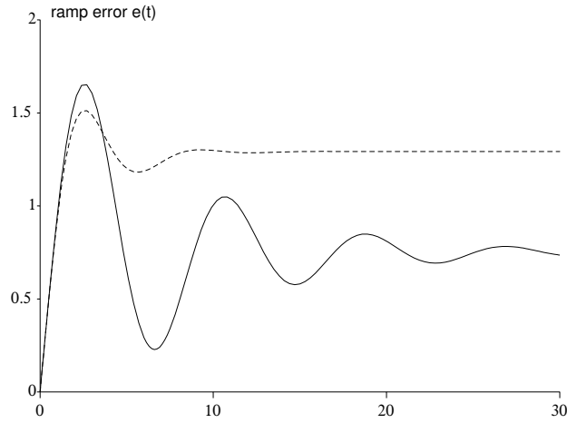
Figure 6.14 Ramp error of the uncompensated closed loop system (solid line) as well as the compensated closed loop system (dashed line) in assignment 6.15.
