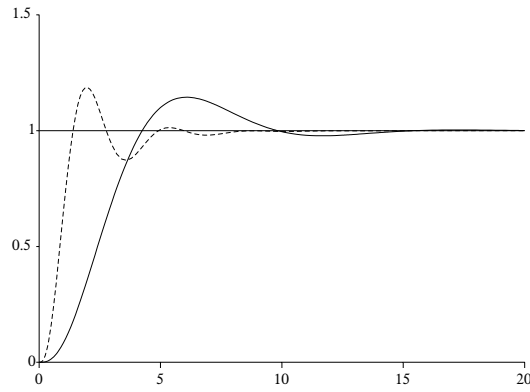
Figure 6.10 The step response of the uncompensated closed loop system (solid line) as well as the compensated closed loop system (dashed line) in assignment 6.14.
