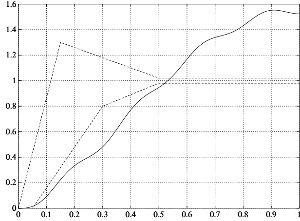
Figure 8.2 The step response with PID control according to Ziegler-Nichols.
