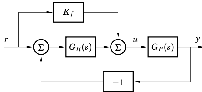
Figure 7.3 Block diagram showing assignment 7.3.
