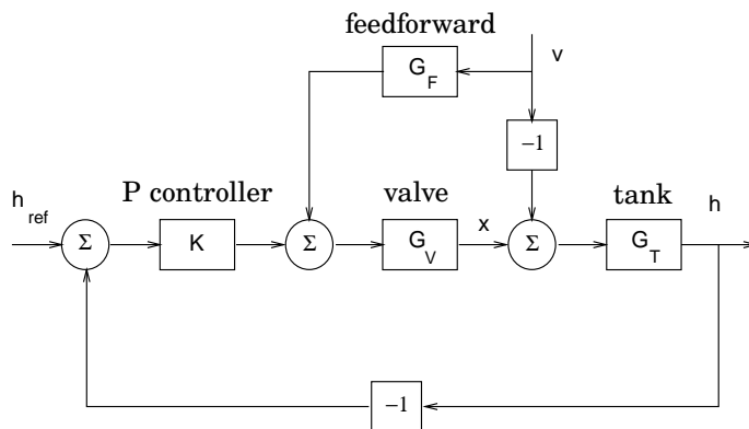
Figure 7.1 Block diagram of the level controlling system in assignment 7.2.
