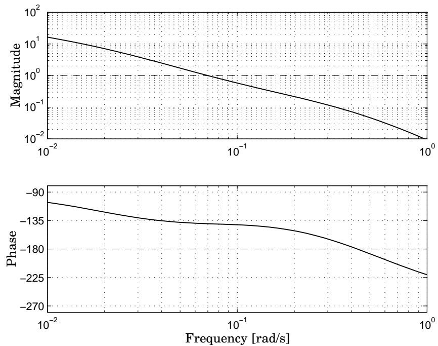
Figure 4.6 Bode plot of the open loop transfer function of the controlled lower tank in the double tank process in problem 4.19.
