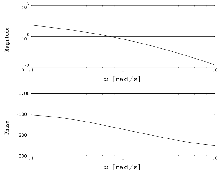
Figure 6.12 Bode plot of G_o(s) in assignment 6.15.
