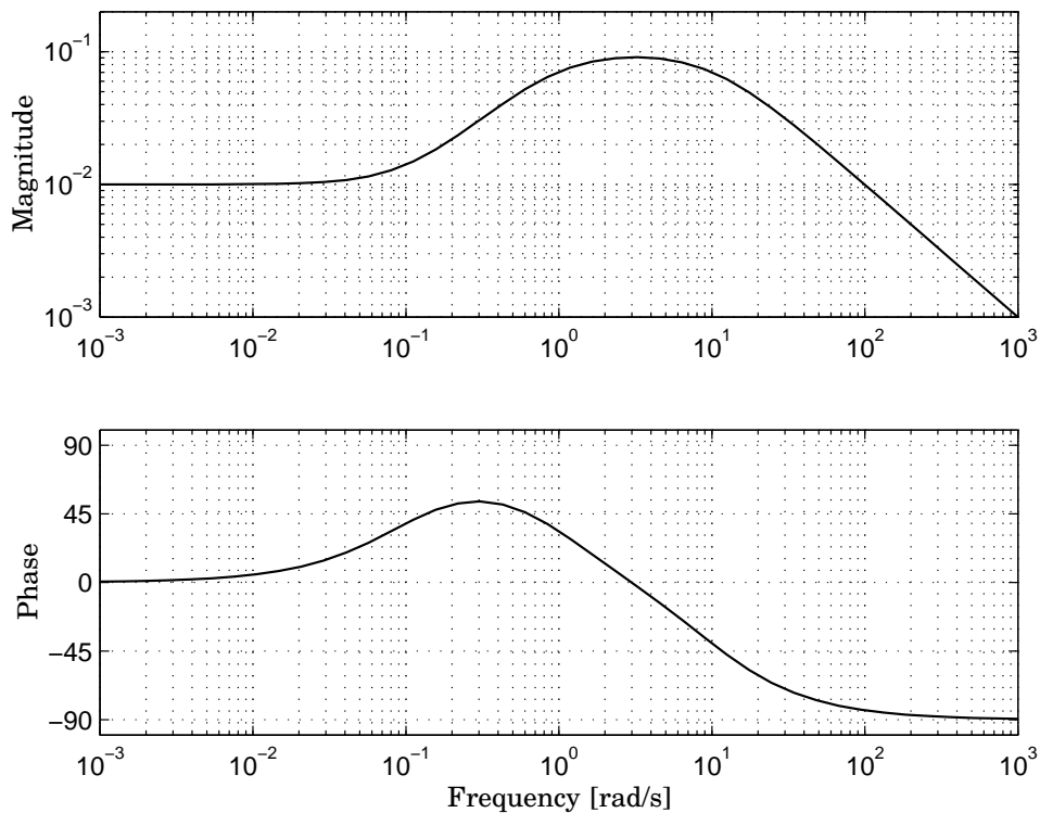
Figure 3.1 The Bode plot in assignment 3.1.
