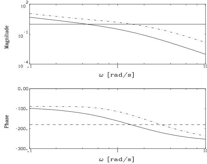
Figure 6.9 Bode plot of the uncompensated system G_1 (solid line) and compensated system G_k G_1 (dash-dotted line) in assignment 6.14.
