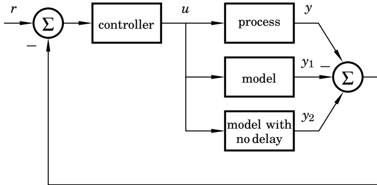
Figure 7.7 Working principle of the Smith predictor.
