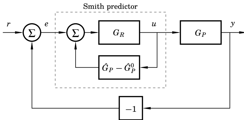
Figure 7.8 Block diagram equivalent to Figure 7.7.
