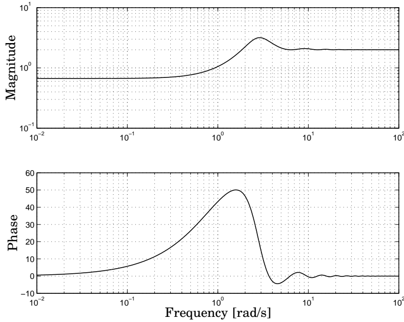
Figure 7.3 Bode plot of the Smith predictor.
