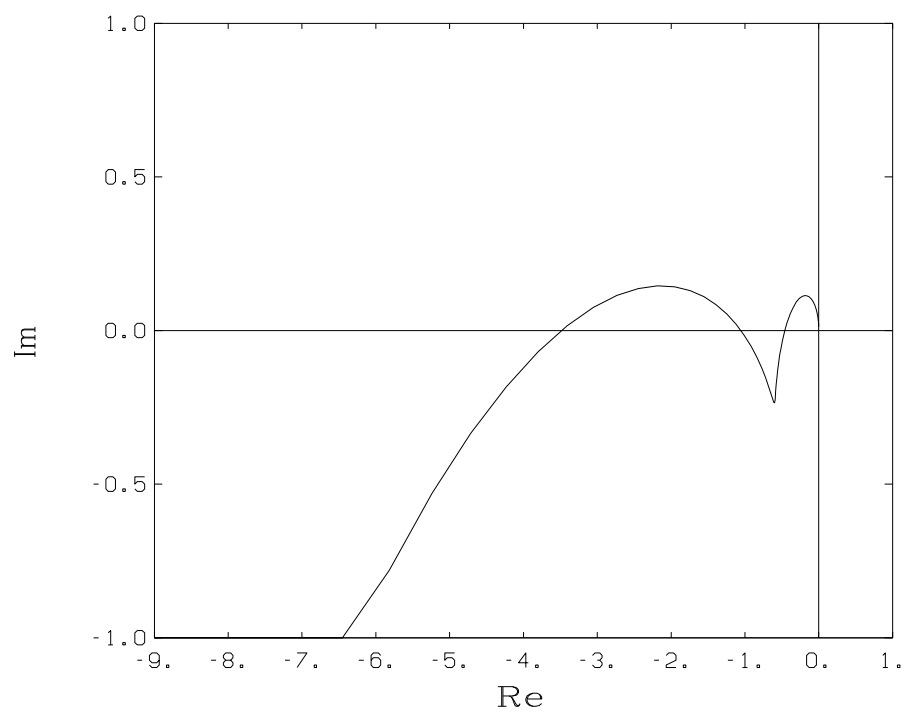
Figure 4.2 Nyquist curve of the system in assignment 4.14.
