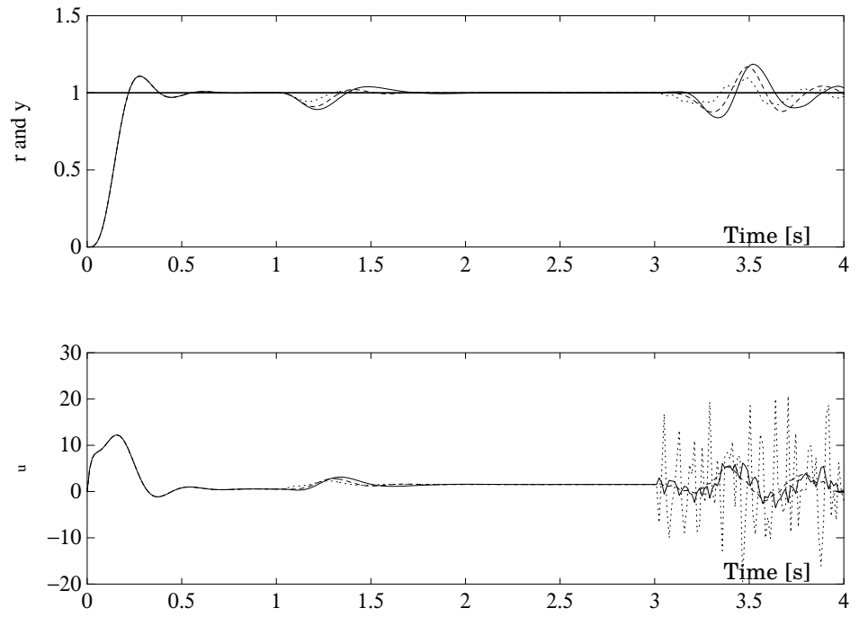
Figure 8.11 Evaluation of control with \omega_m = 20 and \omega_o = 10 (solid curves), 20 (dashed curves) and 40 (dotted curves).
