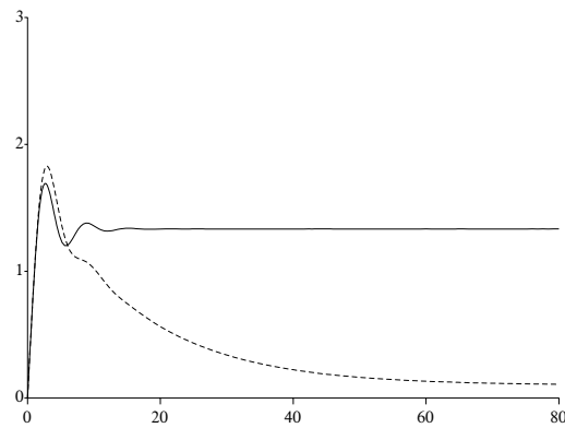
Figure 6.17 Ramp error of the uncompensated closed loop system (solid line) as well as the compensated closed loop system (dashed line) in assignment 6.16.
