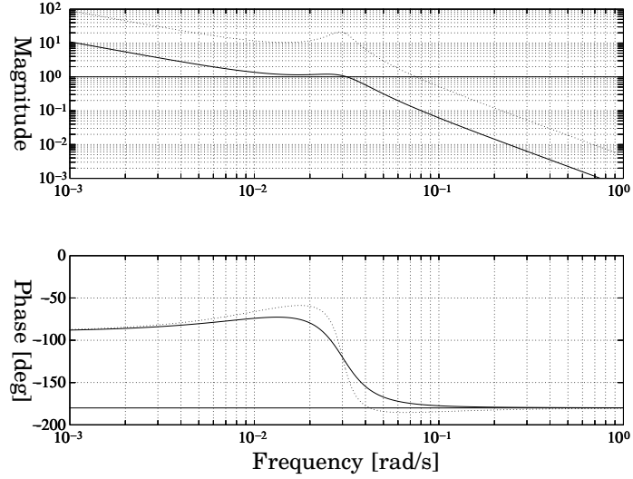
Figure 8.1 Bode plot of the PD compensated open loop system in assignment 8.1. The solid curves show the case v = 7 knots. Note that the latter case yields an unstable closed loop system.
