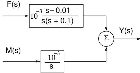
Figure 7.6 Block diagram of steam boiler with dome.
