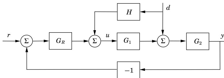
Figure 7.1 Block diagram of the temperature control system in a house.
