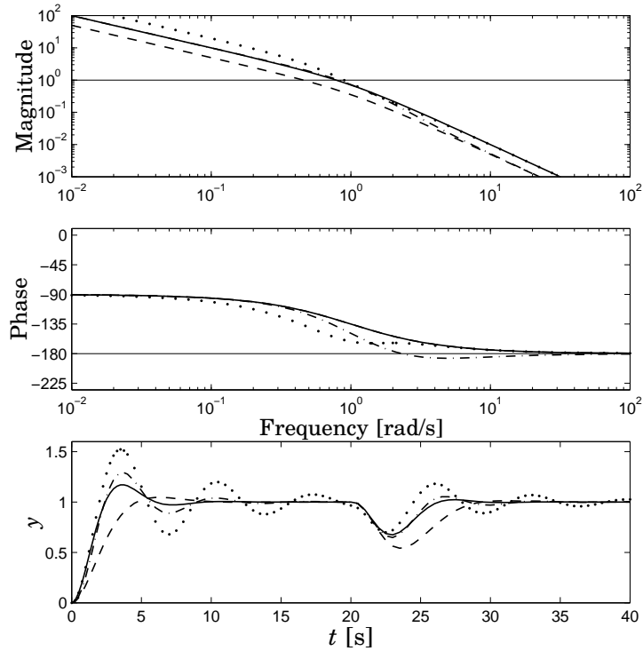
Figure 6.2 Bode plot and step response for the case when the PID parameters in sub-assignment 6.2b have been divided by two. The solid curves correspond to the nominal case.
