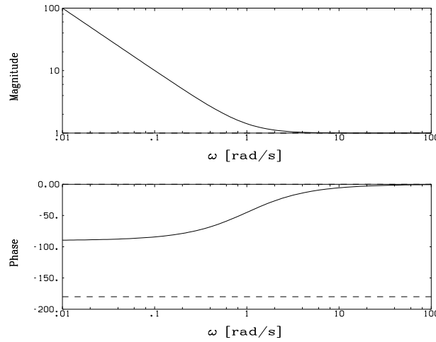
Figure 6.1 Bode plot of a PI controller with K = 1 and T_i = 1 .
