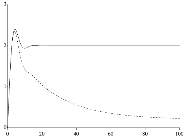
Figure 6.6 Ramp error of the uncompensated system (solid line) as well as the compensated system (dashed line) in assignment 6.12.
